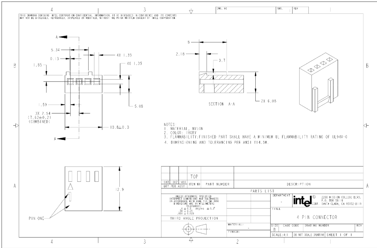
Figure 7 Connector Housing
