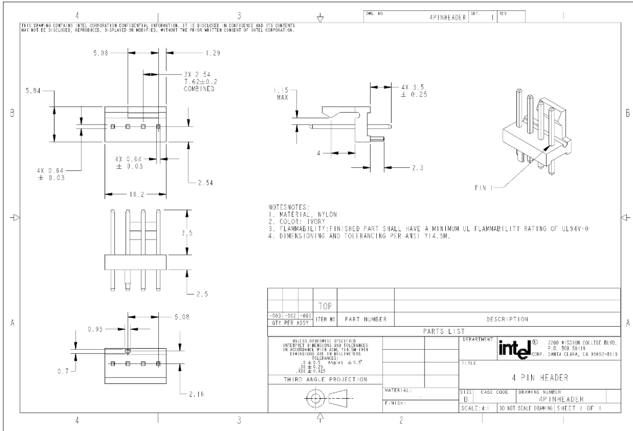
Figure 8 Baseboard Connector
