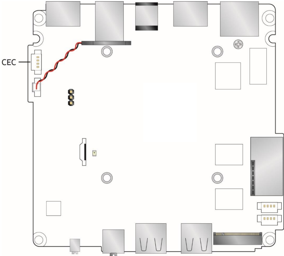
Figure 8. CEC Connector
