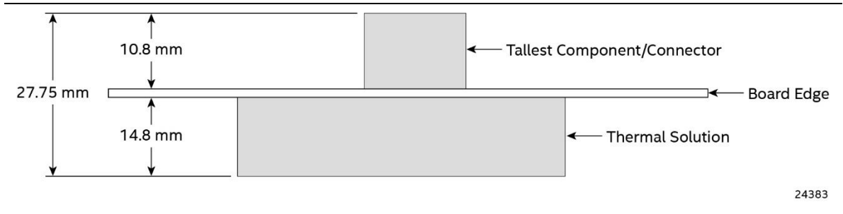
Figure 16. Board Height Dimensions
