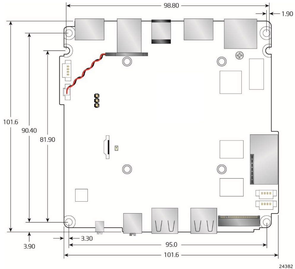
Figure 15. Board Dimensions
