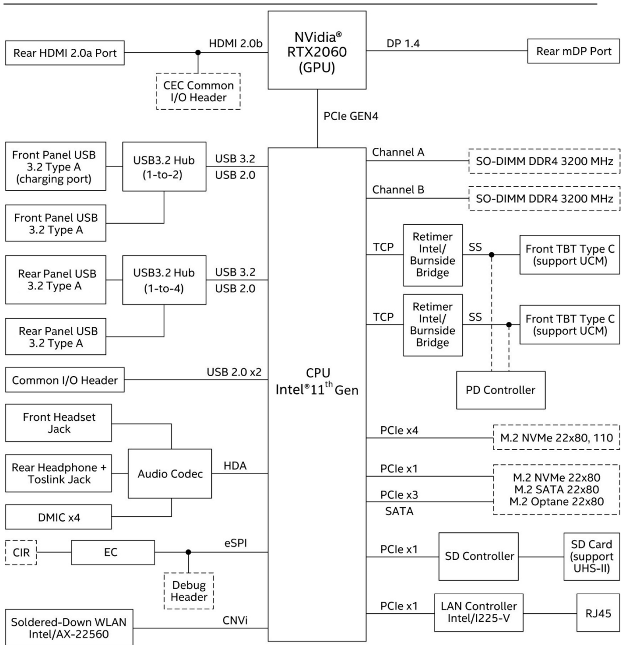
Figure 4. Block Diagram
