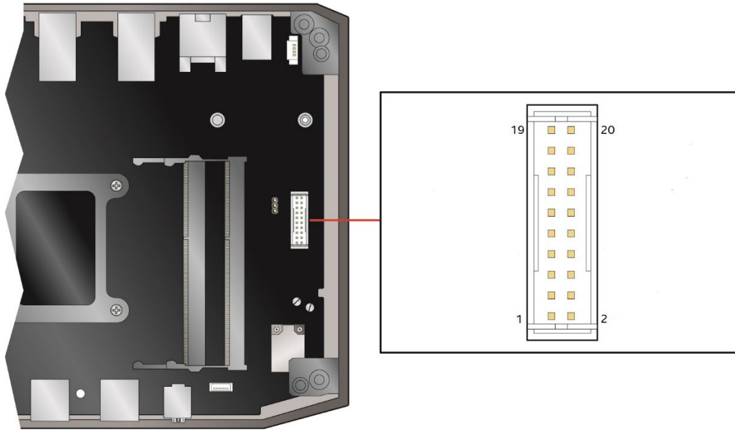
Figure 6. Common IO Header (1.25 mm Pitch)
