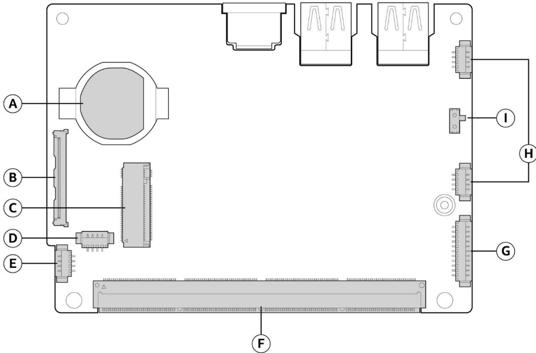
Figure 2. Features (Top)
