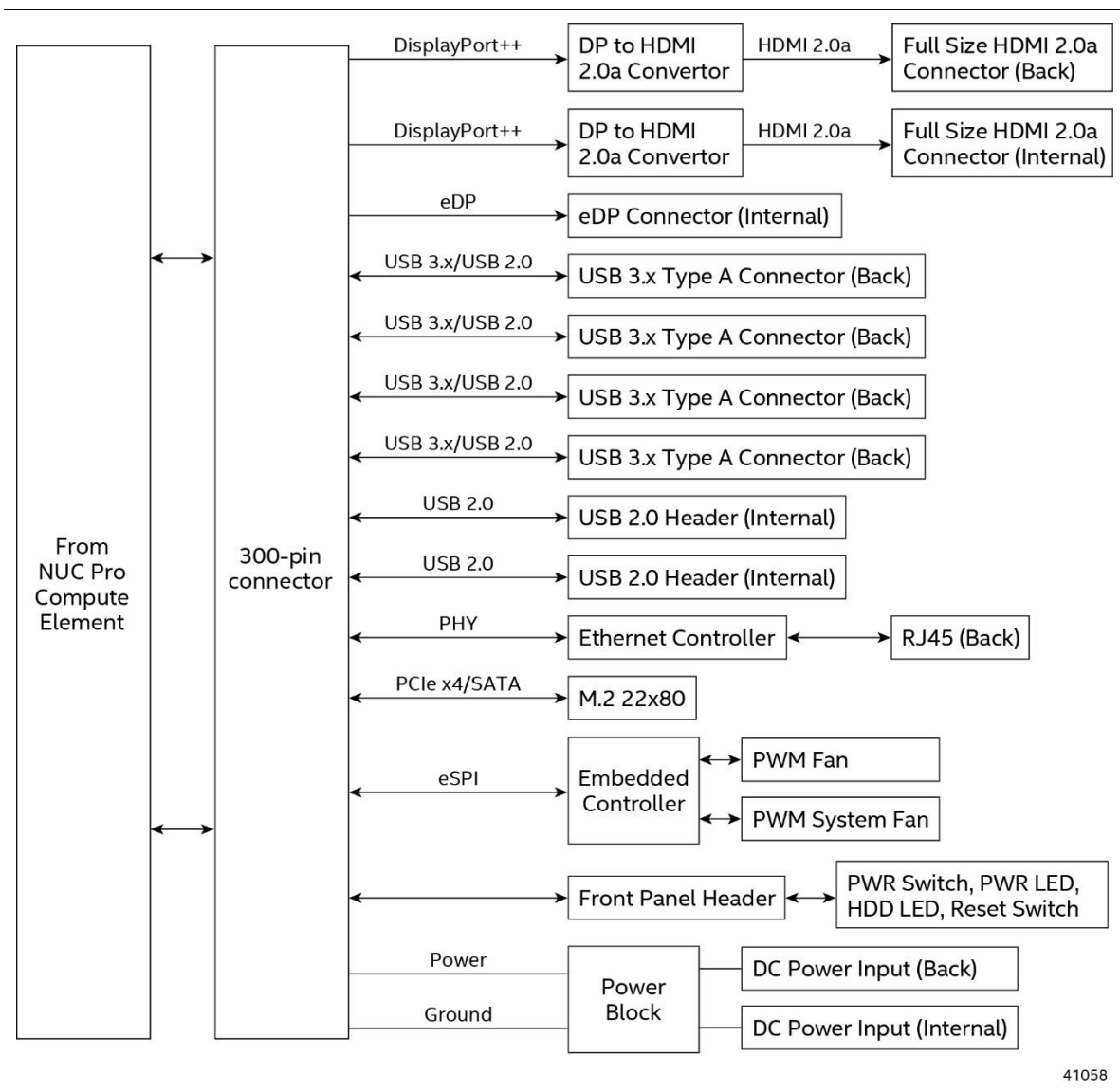
Figure 1. Block Diagram
