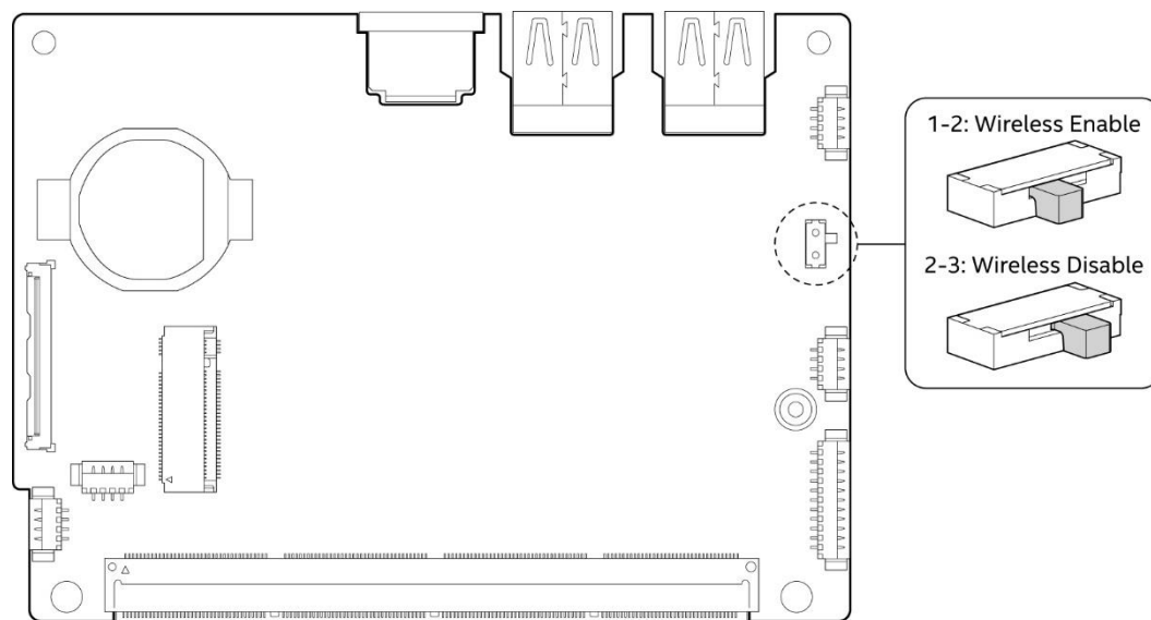
Figure 4. Wireless Enable/Disable Switch Location
